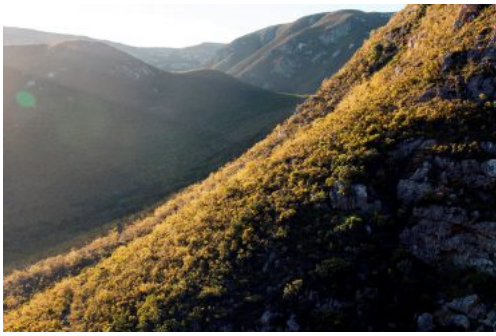
Our approach
